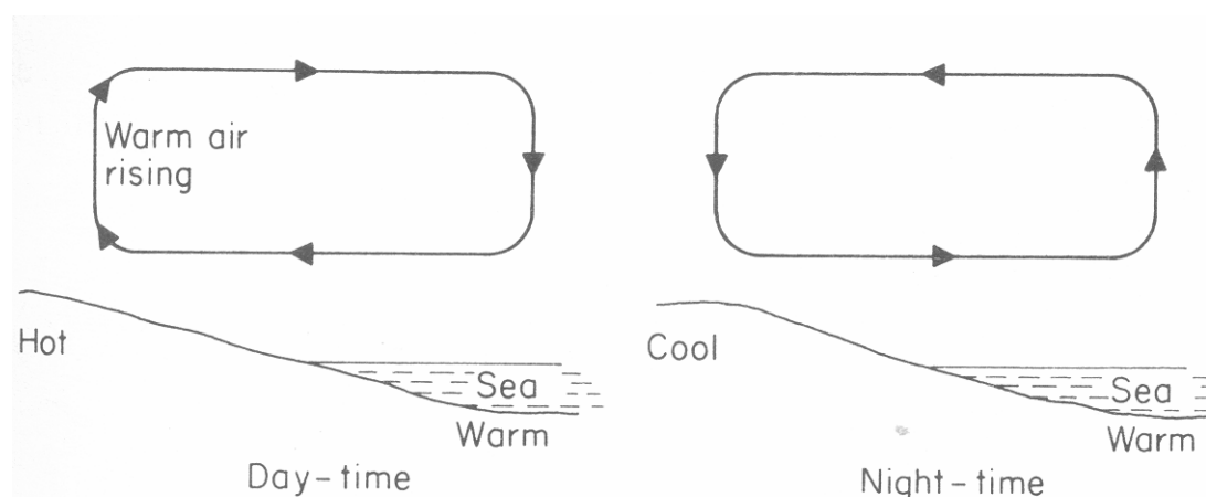
Fig. 17.15. Land and sea breezes
