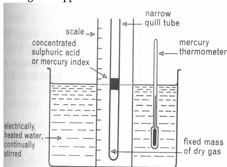
Fig. 5.9 Charles's Law
