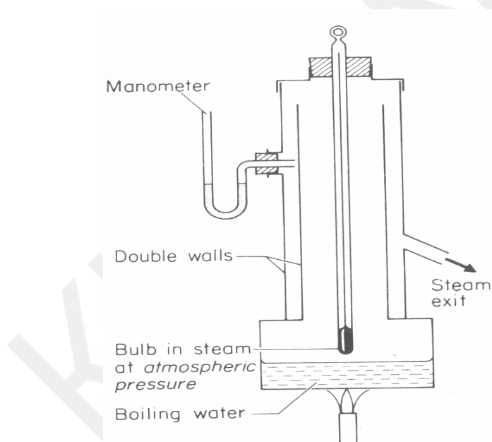
Fig. 14.2. Hypsometer (upper fixed point)
