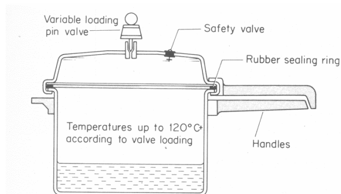
Fig. 20.5. Pressure cooker
