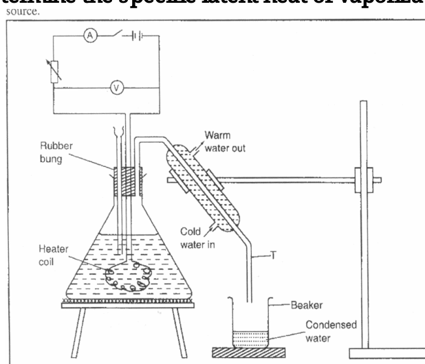
Fig. 9.13: Determining specific latent of vaporisation of water using electrical method
